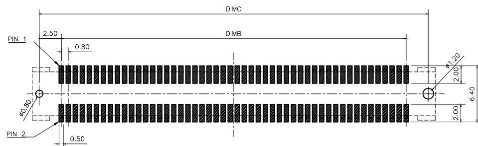
RECOMMEND PCB LAYOUT TOLERANCE±0.05mm
